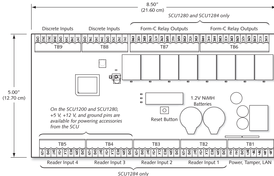
Figure 1. SCU Controller
